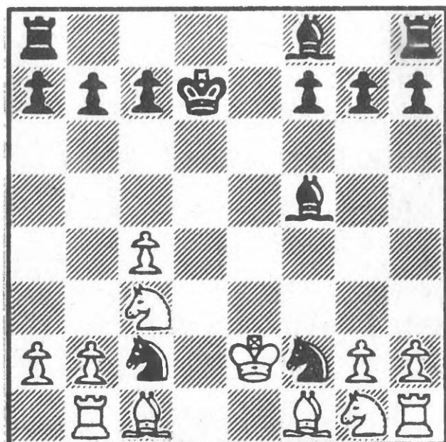
54 After 14 Ke2
